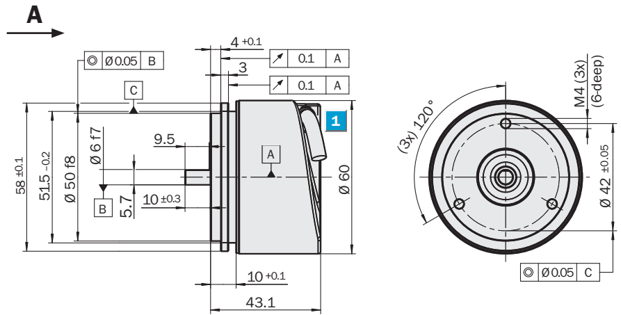
Dimensional drawing servo flange, cable outlet
