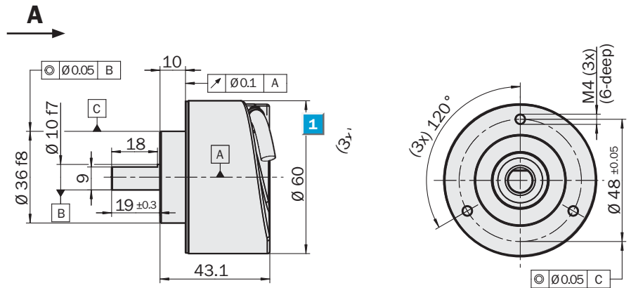
Dimensional drawing face mount flange, cable outlet
