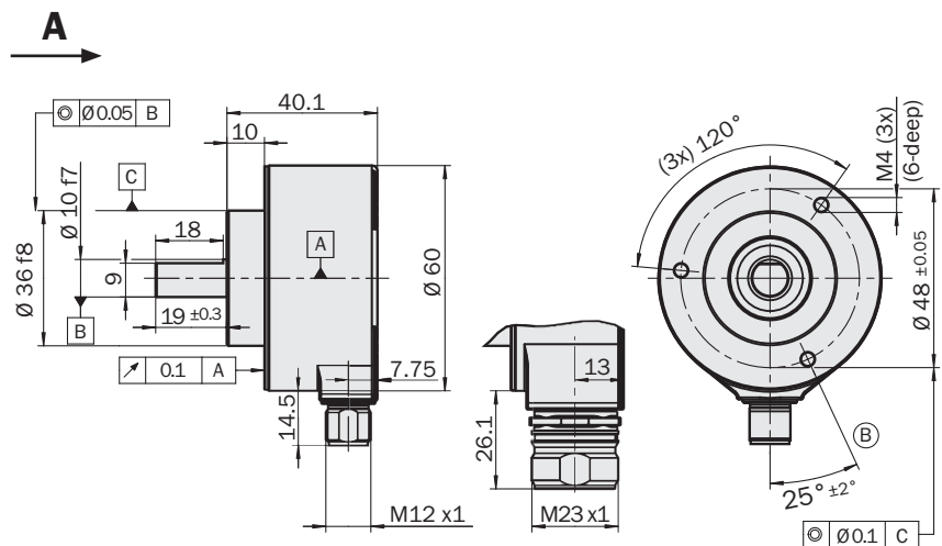
Dimensional drawing face mount flange, connector outlet M12 and M23
