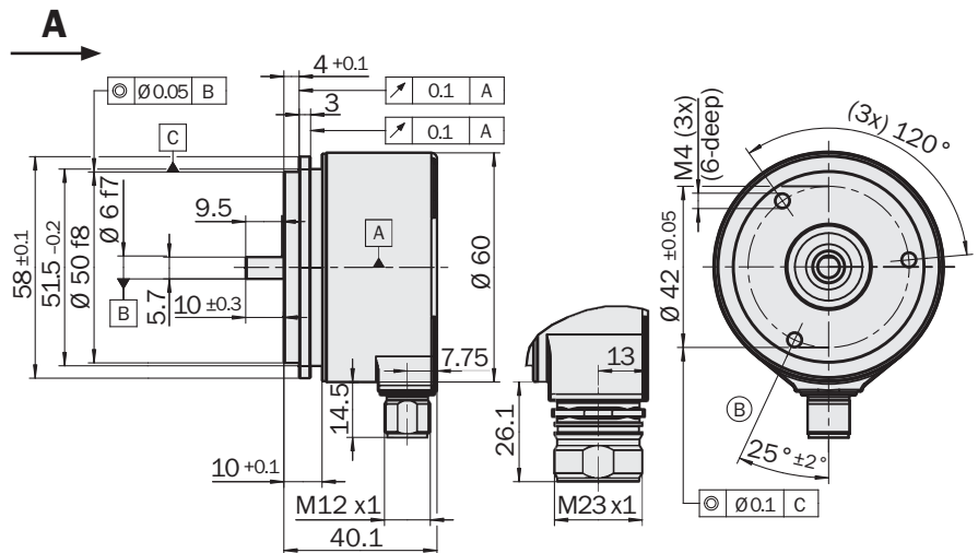
Dimensional drawing servo flange, connector outlet M12 and M23
