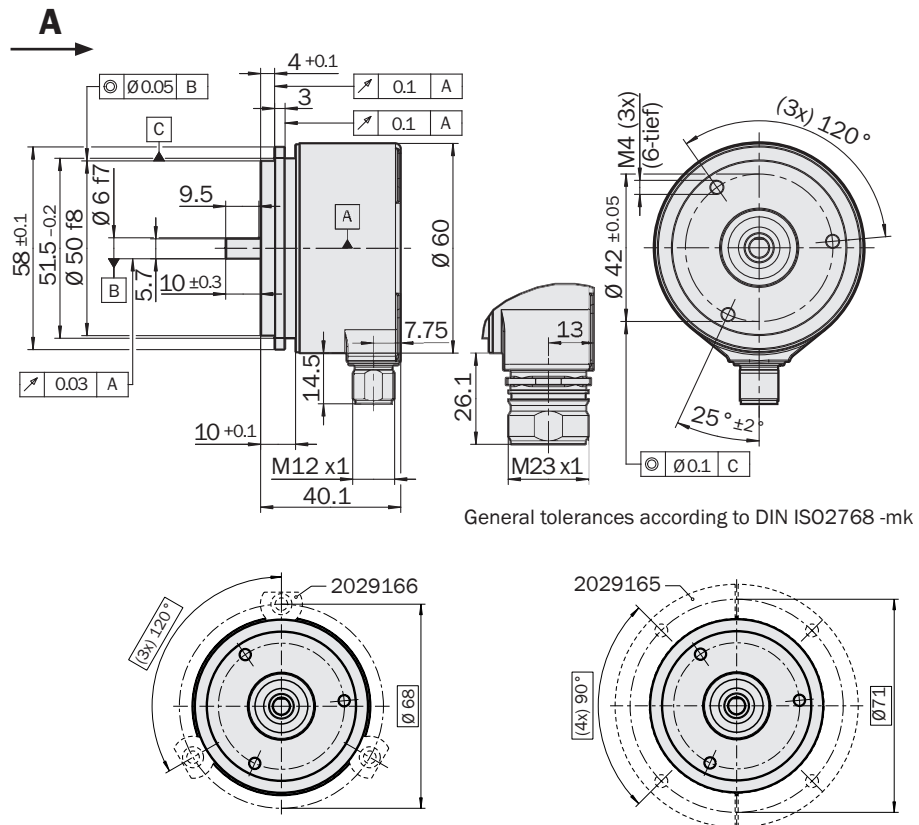
Dimensional drawing servo flange, connector outlet M12 and M23
