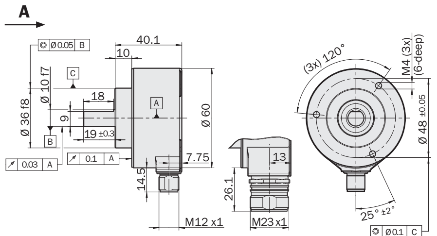
Dimensional drawing face mount flange, connector outlet M12 and M23
