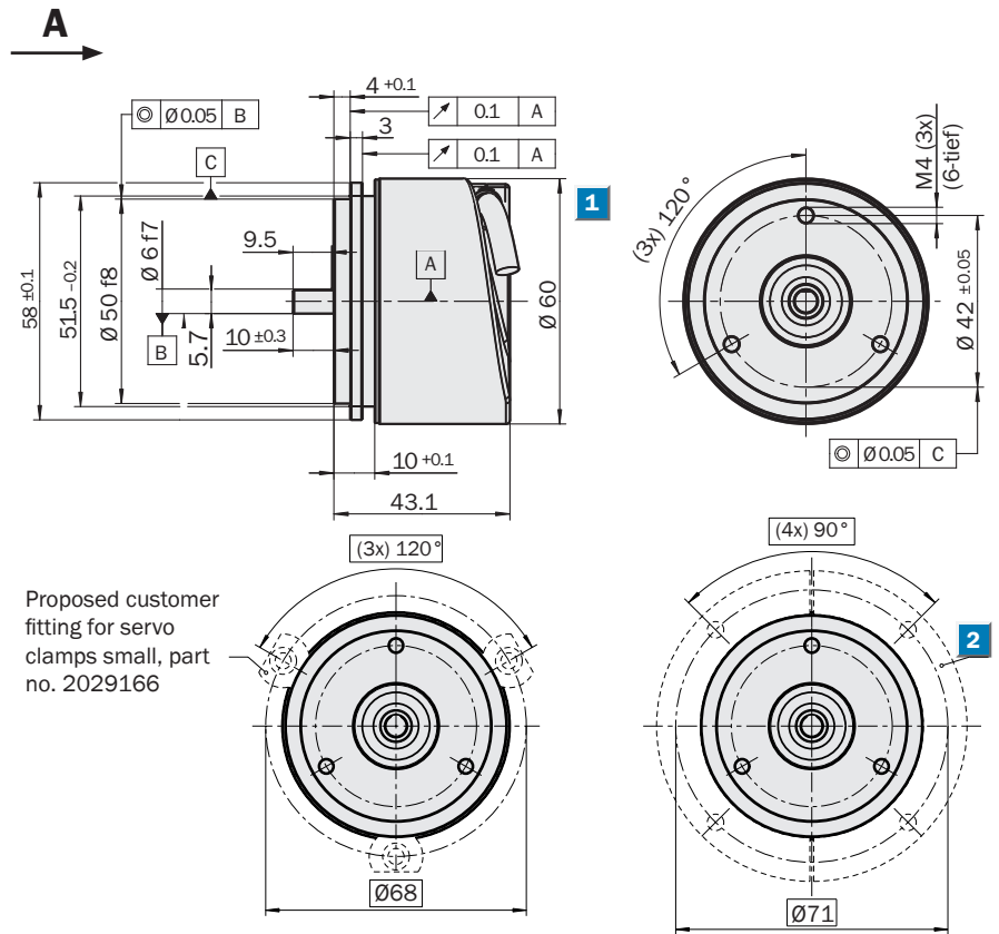
Dimensional drawing servo flange, cable outlet
