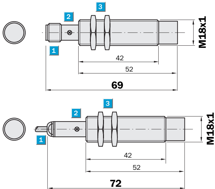
Dimensional drawing
