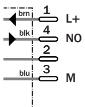
M12, 4-pin
