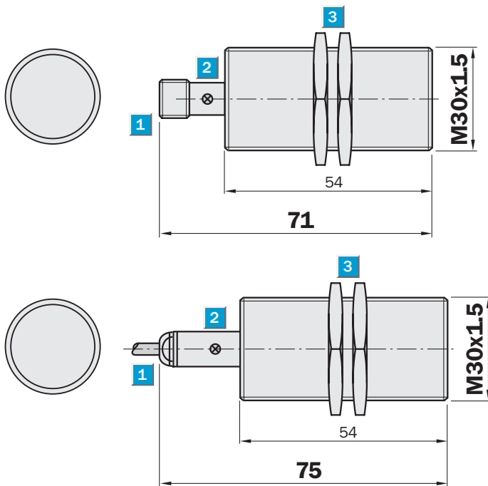
Dimensional drawing
