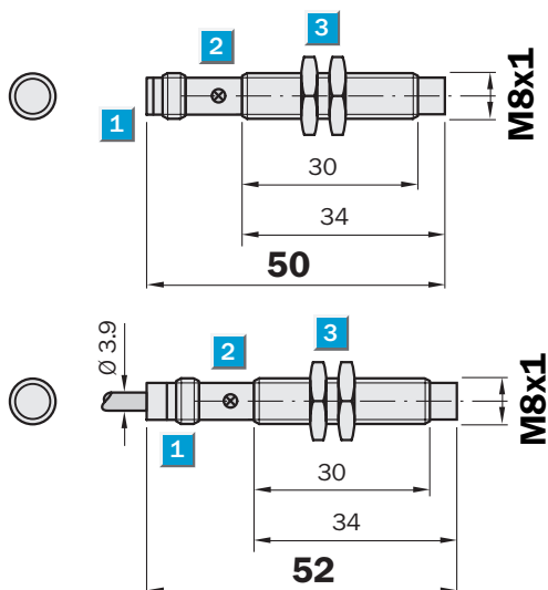
Dimensional drawing
