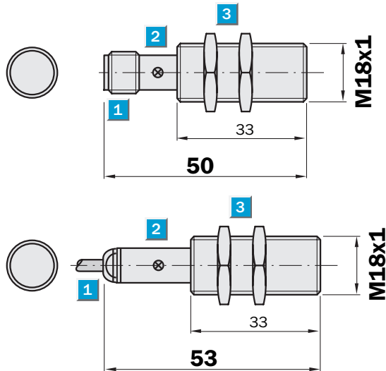
Dimensional drawing
