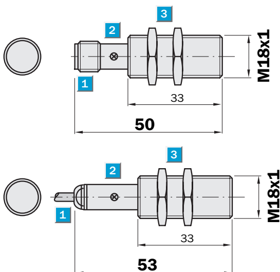
Dimensional drawing
